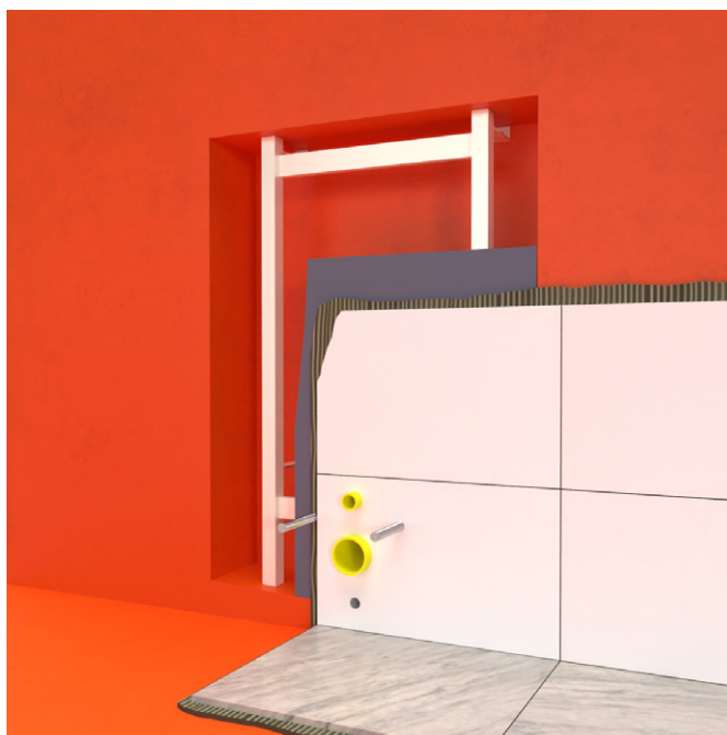
FIGURE 23. Watertight membrane behind built-in WC in wall
